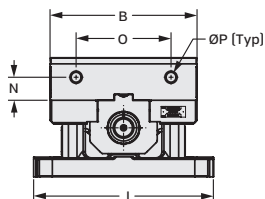
End View
