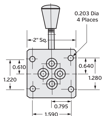
Manifold Mount Model
