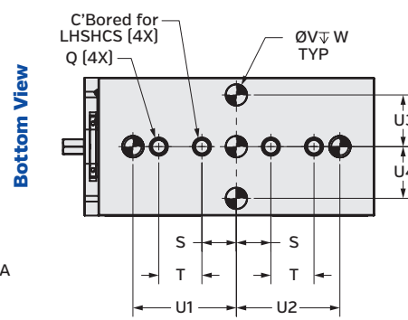
Riser Not Shown in This View
