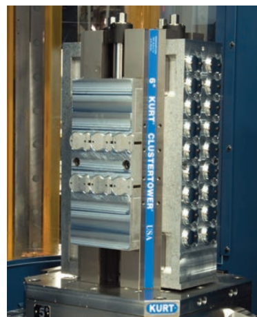
Cluster Tower using fixture plate & Soft jaws
