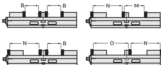
Hardened Jaw Positions (Manual Vise Shown)
