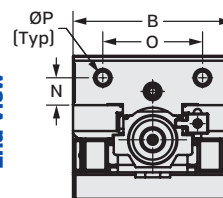
End View
