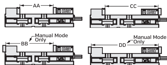
Jaw Position
