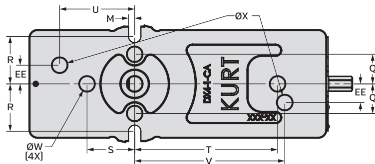
Bottom View
