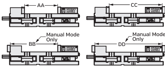
Jaw Position
