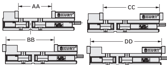
Jaw Position
