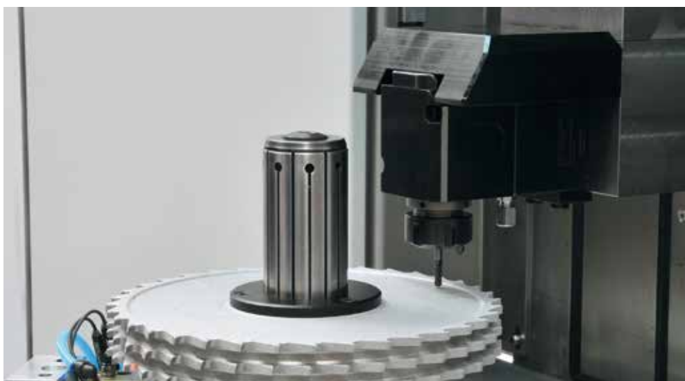
Balancing of PCD jointing cutters for laminate
