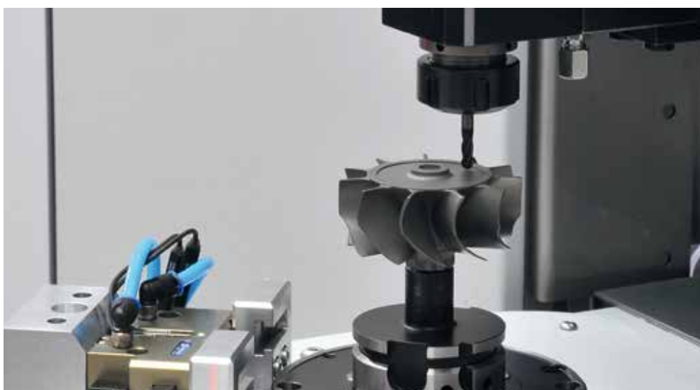
Compressor wheel for turbo charger
