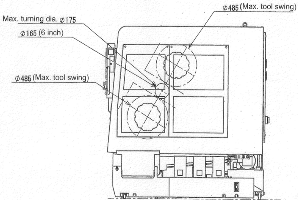
SuperNTY 3 - Tool swing -
