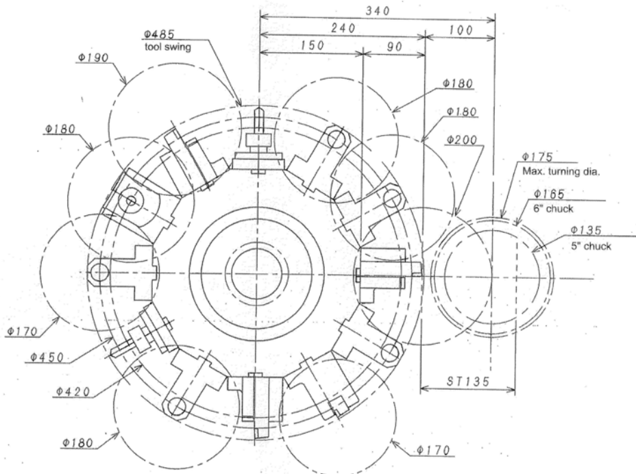
SuperNTY 3 - Tooling interference - 12st
