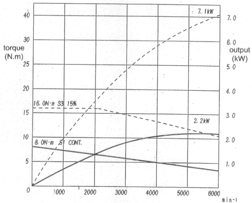
SuperNTY 3 - Speed/Torque/Output - Rotating tool
