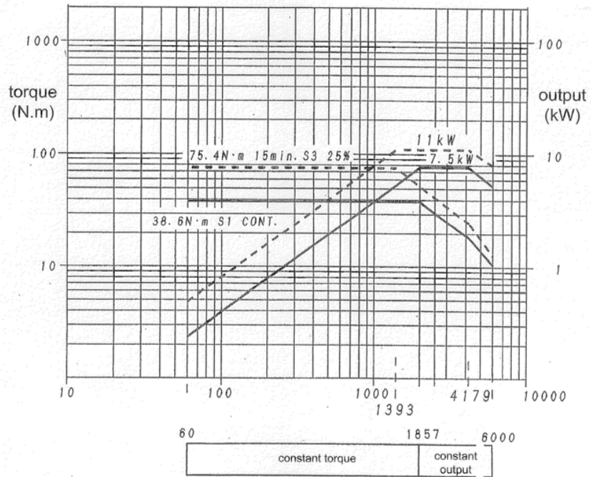
SuperNTY 3 - Speed/Torque/Output - L/R spindle
