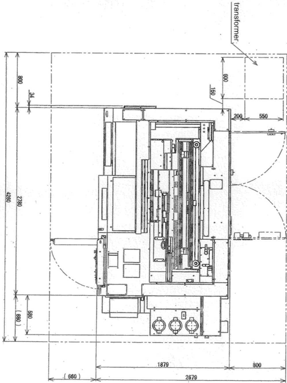
SuperNTY 3 - Floor space - with HP coolant pumps
