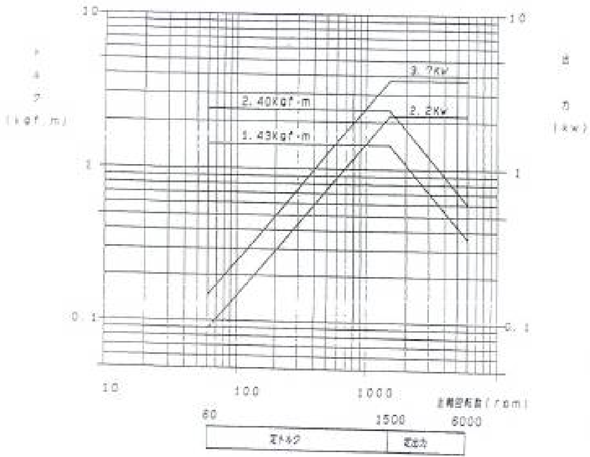
Milling motor speed-torque output space (Frame 4.9 (17.9kW))
