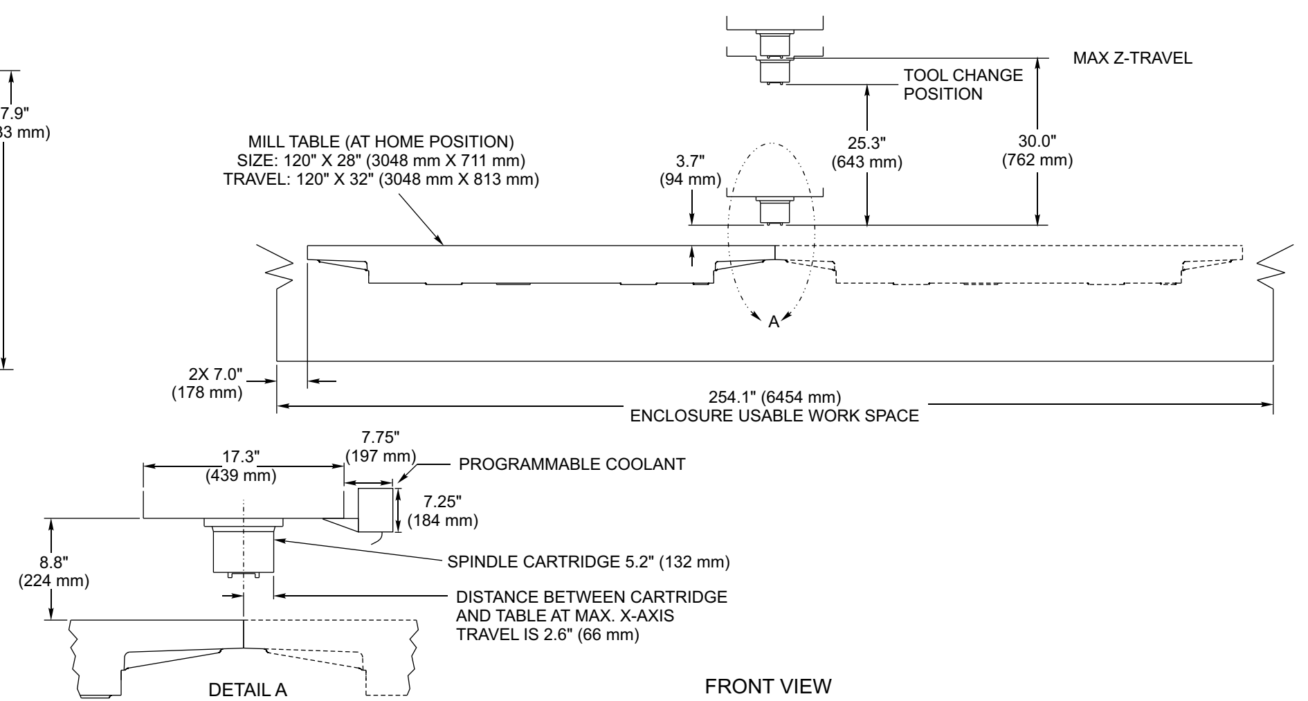
VF-11/40 Enclosure Usable Work Space
