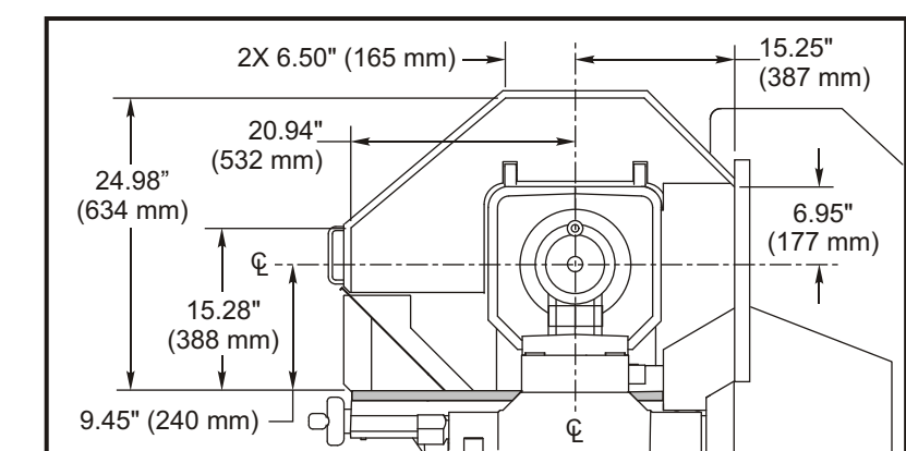
TL-3W Enclosure Work Space (Right Side View)
