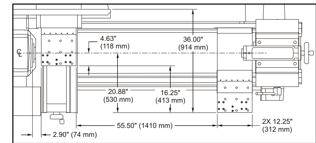
TL-3W Enclosure Work Space (Top View)
