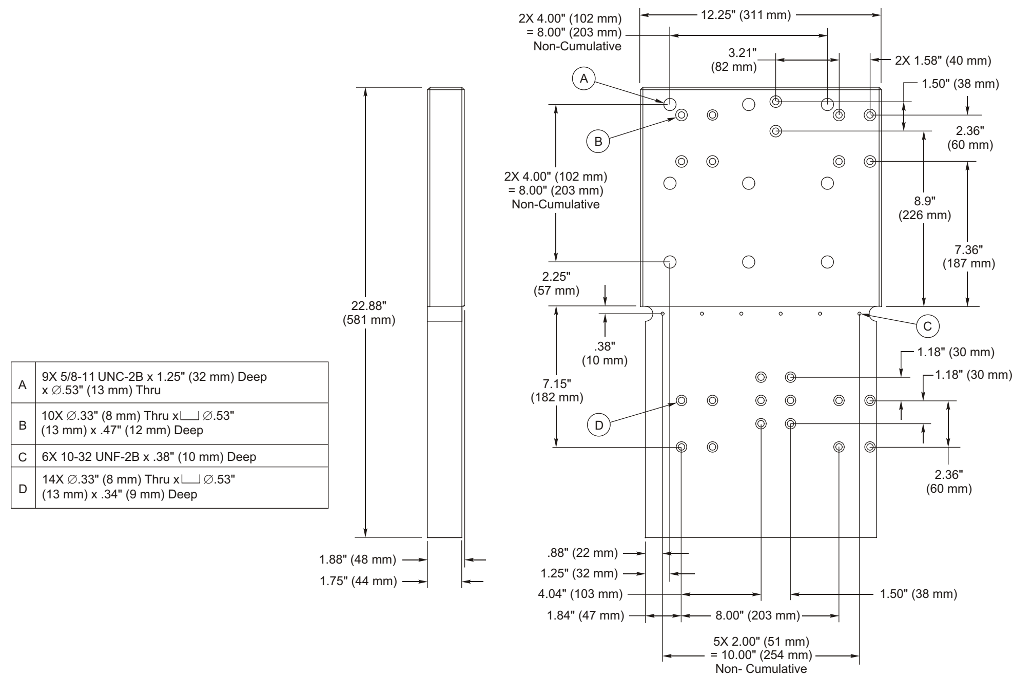
TL-3W Cross Slide Dimensions (View Rotated 180°)
