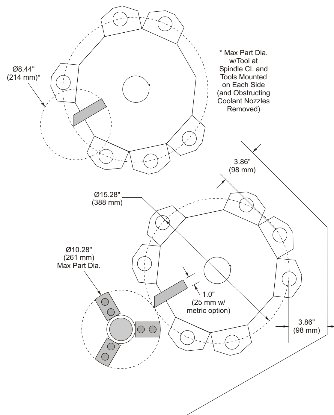
Turret Tooling Clearance - TL-15 with Standard 10-Pocket BOT
