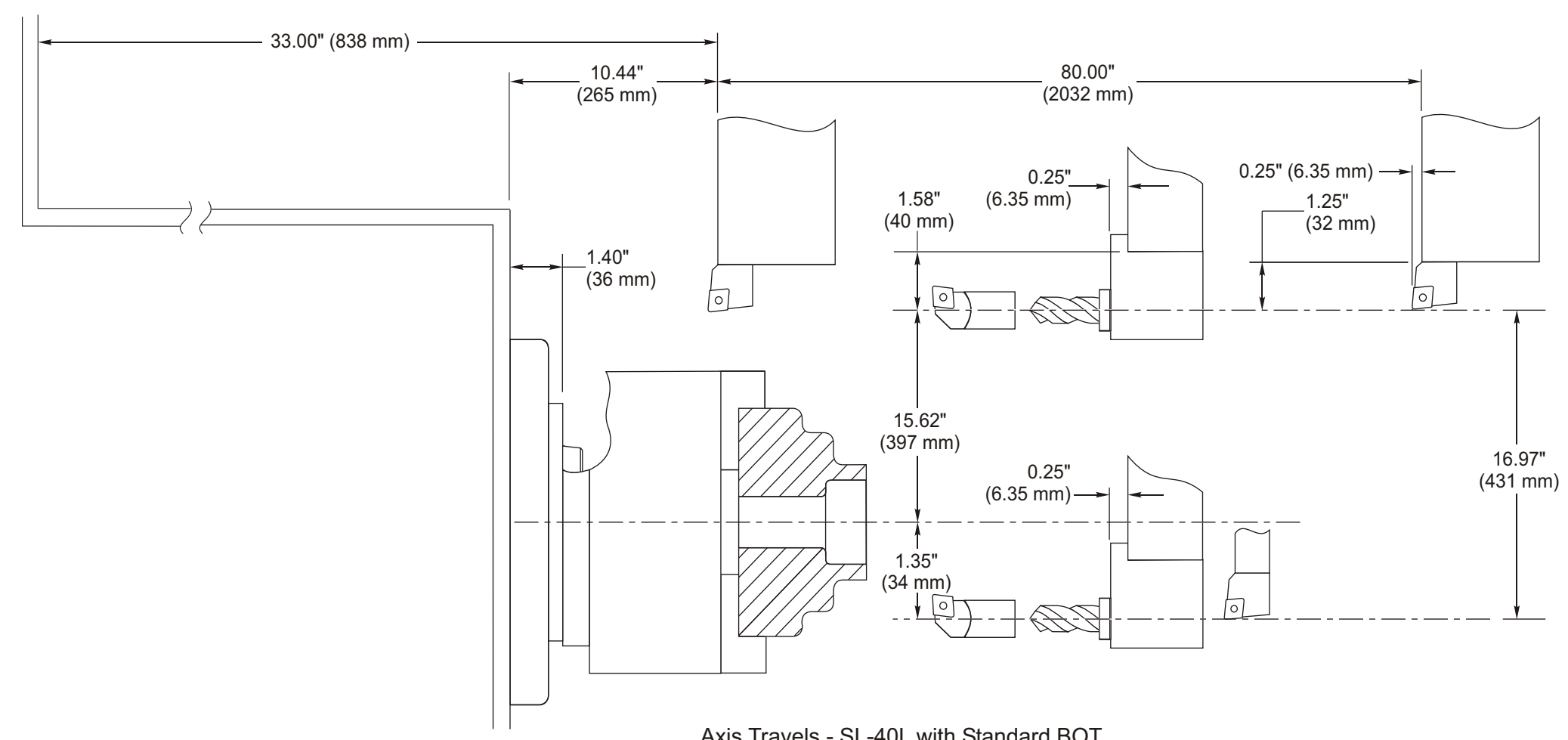
Axis Travels - SL-40L with Standard BOT
