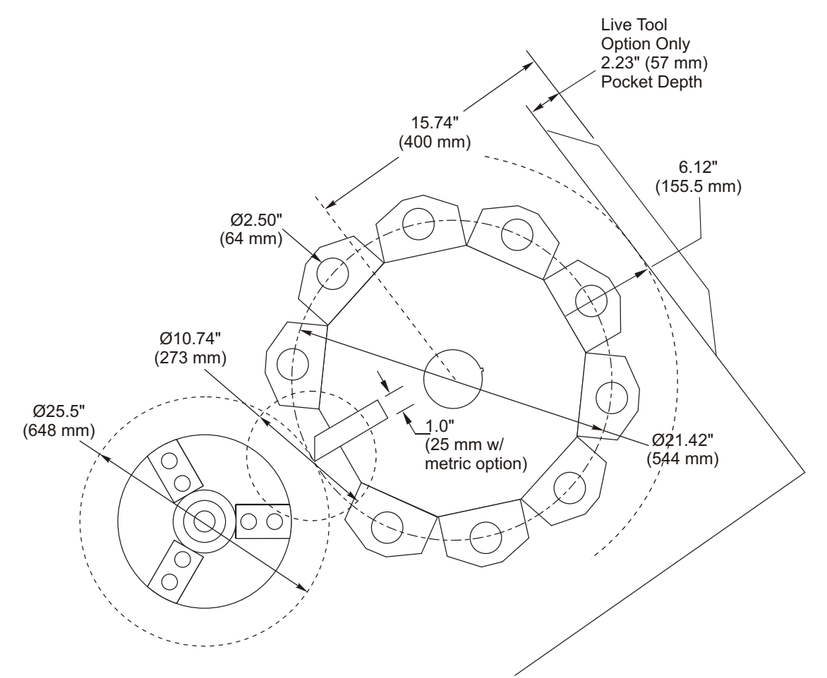
Turret Tooling Clearance - SL-40 with Standard 10-Pocket BOT
