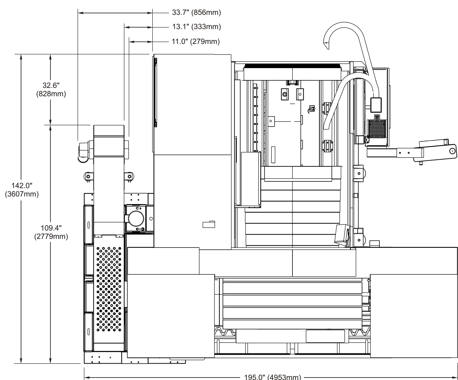
EC-2000 CHIP CONVEYOR DIMENSIONS
