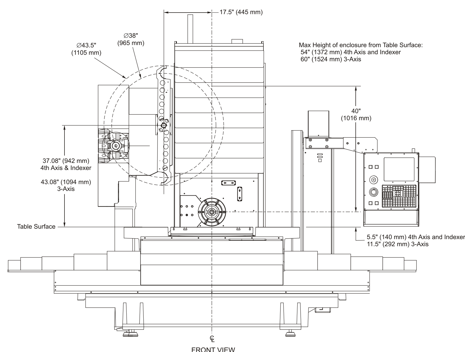
EC-2000 Enclosure Work Space
