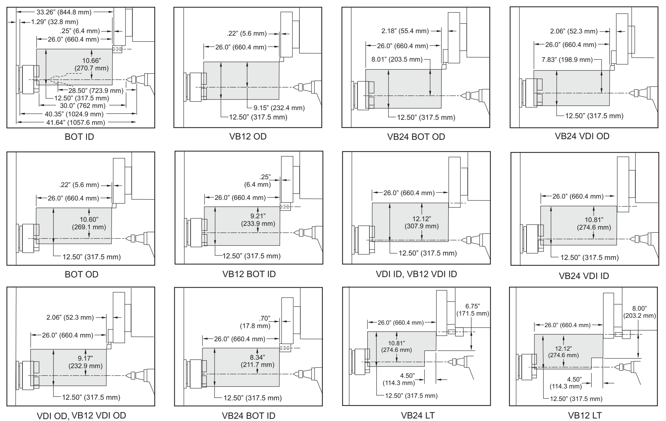
View A-A DS-30 Cut Envelope Diagrams
